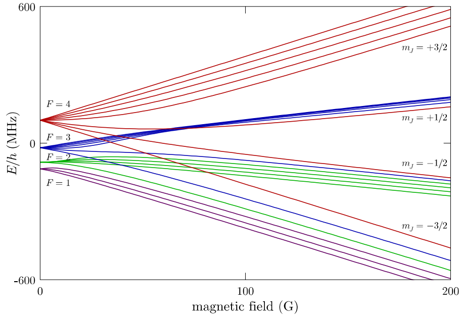
Figure 6: Rubidium 85 5^2P_{3/2} (D 2 excited) level hyperfine structure in an external magnetic field. The levels are grouped according to the value of F in the low-field (Zeeman) regime and m_J in the strong-field (hyperfine Paschen-Back) regime.
